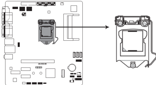
DN-300-R1/R2 CPU socket LGA1151
